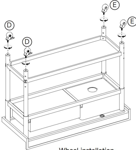
Wheel installation
