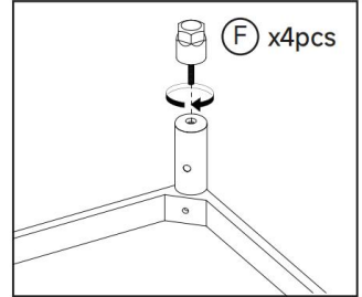
Adjustable foot installation
